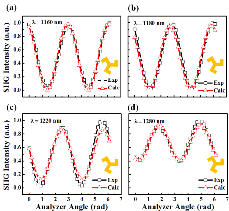
Figure 5. Intensity of the SHG signal as function of the rotation angle of the analyzer for Trisceli-type plasmonic nanostructures. The results are obtained for linearly vertically polarized (V-polarization as shown in Figure 2) illumination at wavelengths of 1160 nm, 1180 nm, 1220 nm and 1280 nm, respectively. The square and triangular symbols represent the measured (Exp) and calculated (Calc) results. By fitting the measured results, we then experimentally determine the second-order effective susceptibilities of SHG from the Trisceli-type nanostructures.
