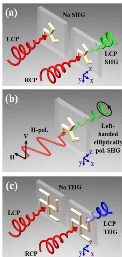
Figure 1. Schematic of nonlinear optical dichroism from Trisceli- and Gammadion- type plasmonic nanostructures with three- (C3) and four-fold(C4) rotational symmetries. (a) and (c) illustrate the nonlinear circular dichroism for illumination with LCP and RCP polarizations on such structures which will lead to SHG and THG with opposite polarizations but only for the RCP illumination. (b) Trisceli-type nanostructures with near unity SHG-CD would generate left-handed elliptically polarized SHG light when illuminated by linear polarized light.
