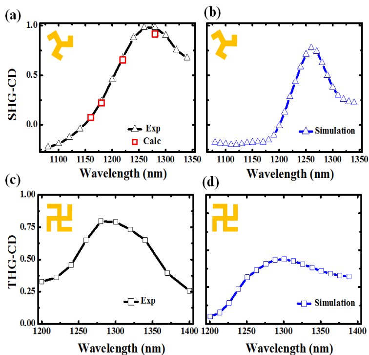
Figure 4. SHG-CD and THG-CD from the Trisceli- and Gammadion- type plasmonic nanostructures. (a) and (c) Measured (Exp) wavelength dependent SHG-CD and THG-CD. The values for the squares in (a) are obtained from the calculation(Calc) of SHG-CD based on the experimentally determined values of the effective nonlinear susceptibilities. Both SHG-CD and THG-CD have a broadband response for fundamental wavelength between 1200 nm and 1350 nm. The SHG-CD experiences a sign change at wavelength of \sim 1150 nm, which is close to the theoretical prediction of 1200 nm.(b) and (d) Corresponding numerically simulated (Simulation) nonlinear CD spectra for the structures. Both of the calculated SHG and THG spectra show similar trend as the measured ones. While the peak of SHG-CD is close to the measured value, the calculated THG has a much higher deviation from our experimental data, which can be attributed to the imperfections of nanofabrication.
